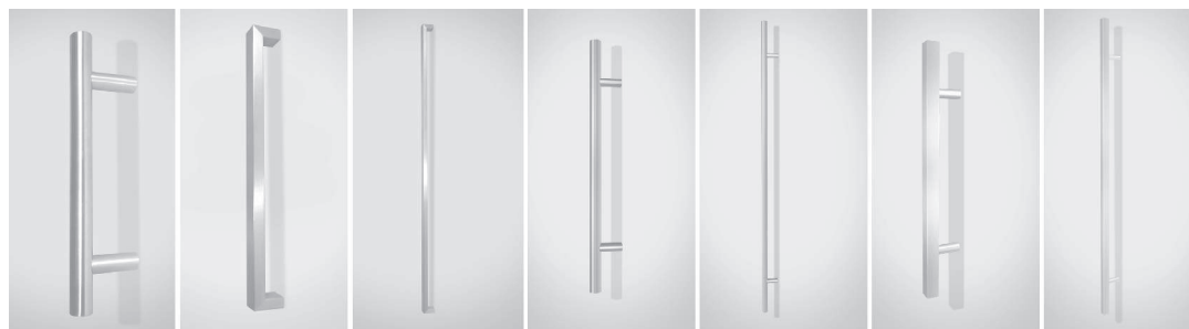
PX01 Ø 25 mm length 300 mm PY01 □ 20 x 40 mm length 500 mm PZ01 □ 20 x 40 mm length 1400 mm PX02 Ø 25 mm length 657 mm PX03 Ø 25 mm length 1500 mm PQ01 □ 30 x 30 mm length 600 mm PQ02 □ 30 x 30 mm length 1400 mm
